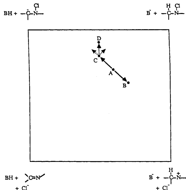
Figure 3. Reaction coordinate energy diagram for base-promoted eliminations from ArCH(R)N(Cl)CH 3 . Points A, B, C, and D represent the transition states for eliminations from ArCH 2 N(Cl)CH 3 , ArCH(Me)N(Cl)CH 3 , and ArCH(Ph)N(Cl)CH 3 in MeONa-MeOH and ArCH(Ph)N(Cl)CH 3 in t -BuOK- t -BuOH, respectively. Contours and transition states for ArCH(Me)N(Cl)CH 3 and ArCH 2 N(Cl)CH 3 in t -BuOK- t -BuOH are omitted. Effects of β-carbon substituents and base-solvent upon the transition states position are shown by solid lines.
