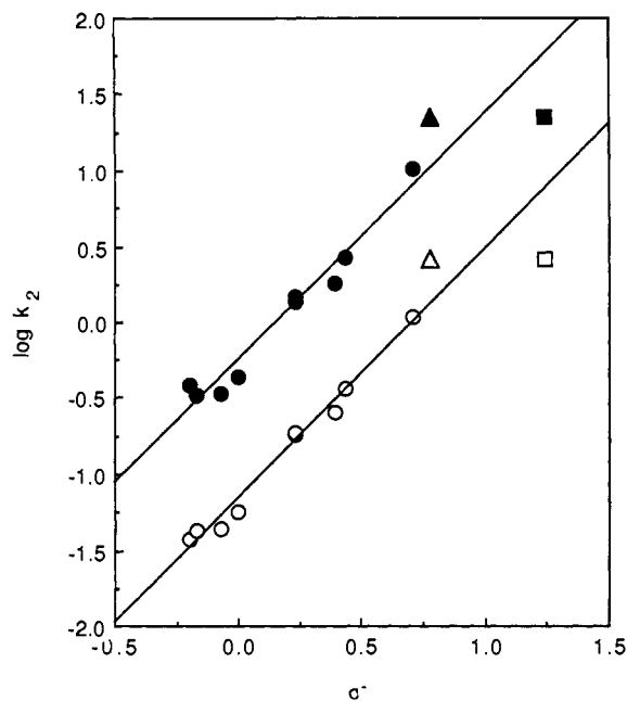
Figure 2. Hammett plots for eliminations from ArCH(Ph)N(Cl)CH_3 promoted by MeONa-MeOH (O) and t -BuOK- t -BuOH (●). (Δ and □ are points for \log k_2 vs \sigma and \sigma' for p -NO 2 , respectively.)
